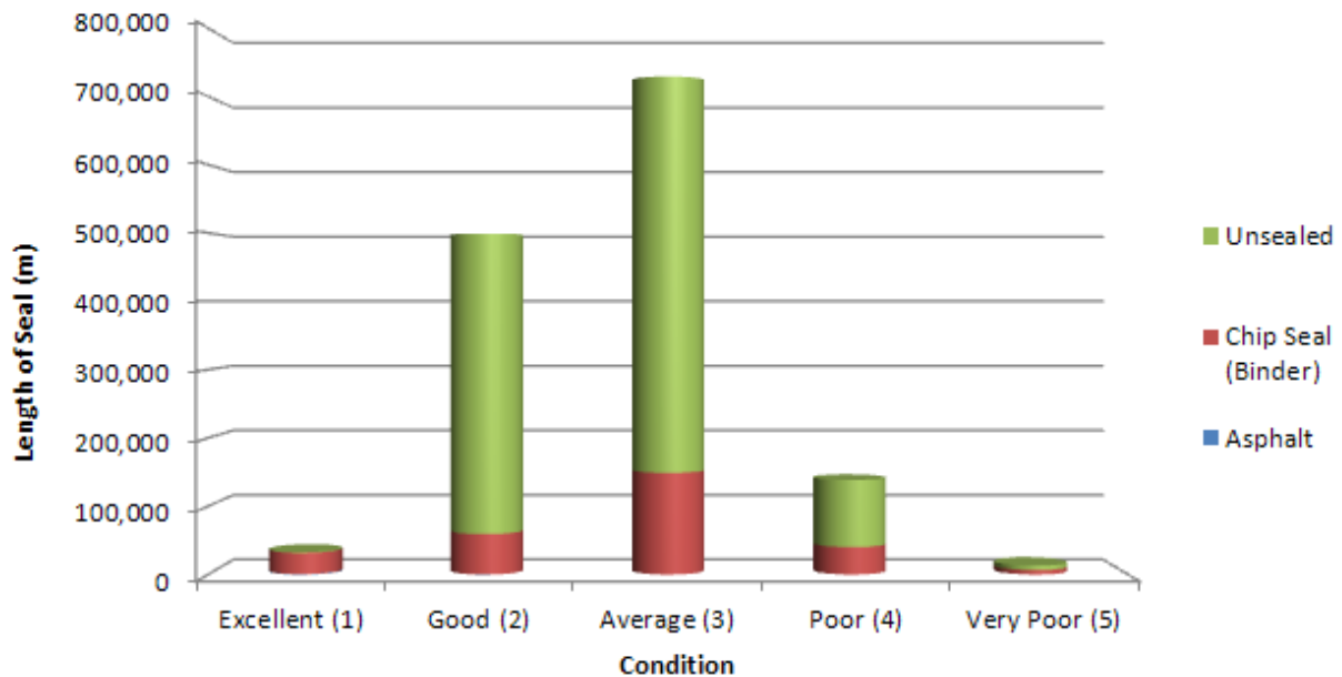
Figure 6-3: Current Road Condition Ratings
